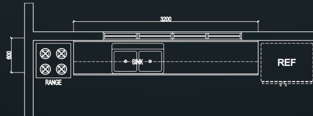
'Magnum' Kitchen Blow-up Plan
