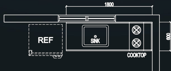
'Magnum' Kitchen Blow-up Plan
